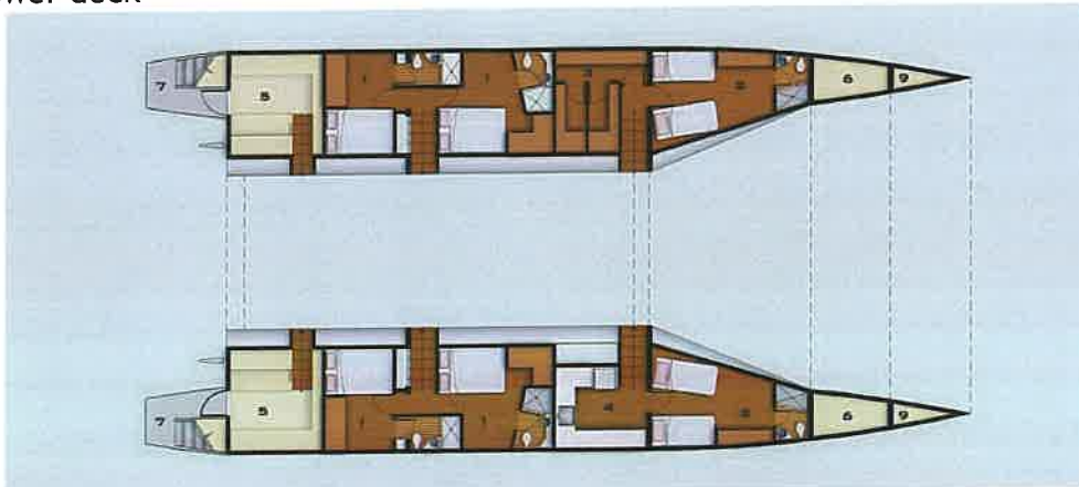
main deck
